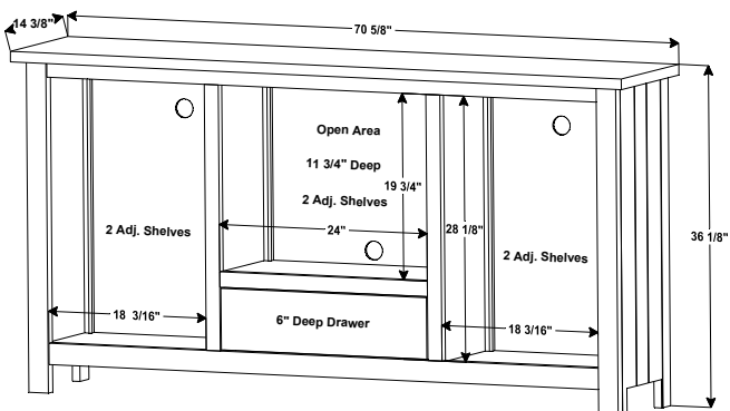
FVE-26-HT (overall size as shown on drawing) FVE-26-A (overall size = 73 1/4"W x 14 7/8"D x 39 1/4"H) FVE-26-BC (overall size = 71 3/8"W x 15"D x 36"H) FVE-26-D (overall size = 70 5/8"W x 14"D x 35 7/8"H) FVE-26-EN (overall size = 73 7/8"W x 14 1/2"D x 38"H) FVE-26-LA (overall size = 72 5/8"W x 15 1/2"D x 36"H)
