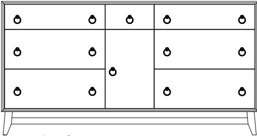
AL-4056 70¾" w 37" h 20" d w/7 drawers, 1 door, 1 adjustable shelf
