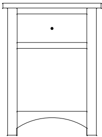
CM-1540 Night Stand 20 3 / 4 "w 27 3 / 4 "h 17 1 / 2 "d w/1 drawer
