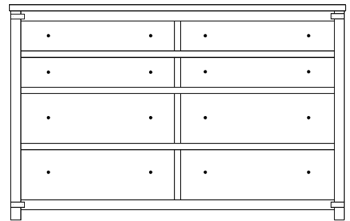
LN-2344 Dresser 67 \frac{1}{4} "w 43"h 19 \frac{3}{4} "d w/8 drawers
