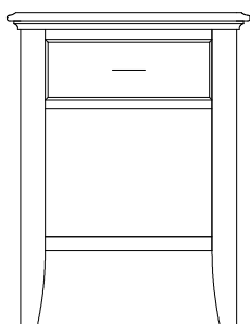
MO-1440 Night Stand 22¼"w 28¾"h 17¾"d w/1 drawer
