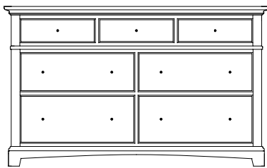
HM-1854 Dresser 60½"w 36½"h 21½"d w/7 drawers
