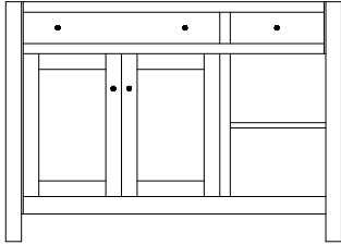
IS-801 47 \frac{3}{4} "w 34 \frac{1}{2} "h 24 \frac{1}{2} "d w/2 drawers 2 doors w/1 adjustable shelf, 1 open shelf
