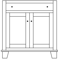
IS-2071 32½"w 34½"h 24"d w/1 drawer 2 doors w/1 adjustable shelf
