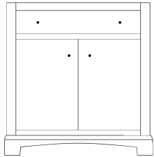
DSB-240 32½"w 34½"h 24½"d w/1 drawer, 2 doors
