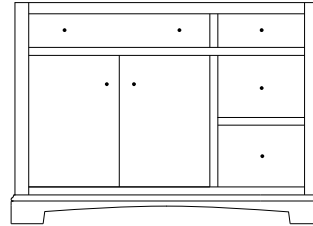
DSB-245 47¼"w 34½"h 24½"d w/4 drawers, 2 doors
